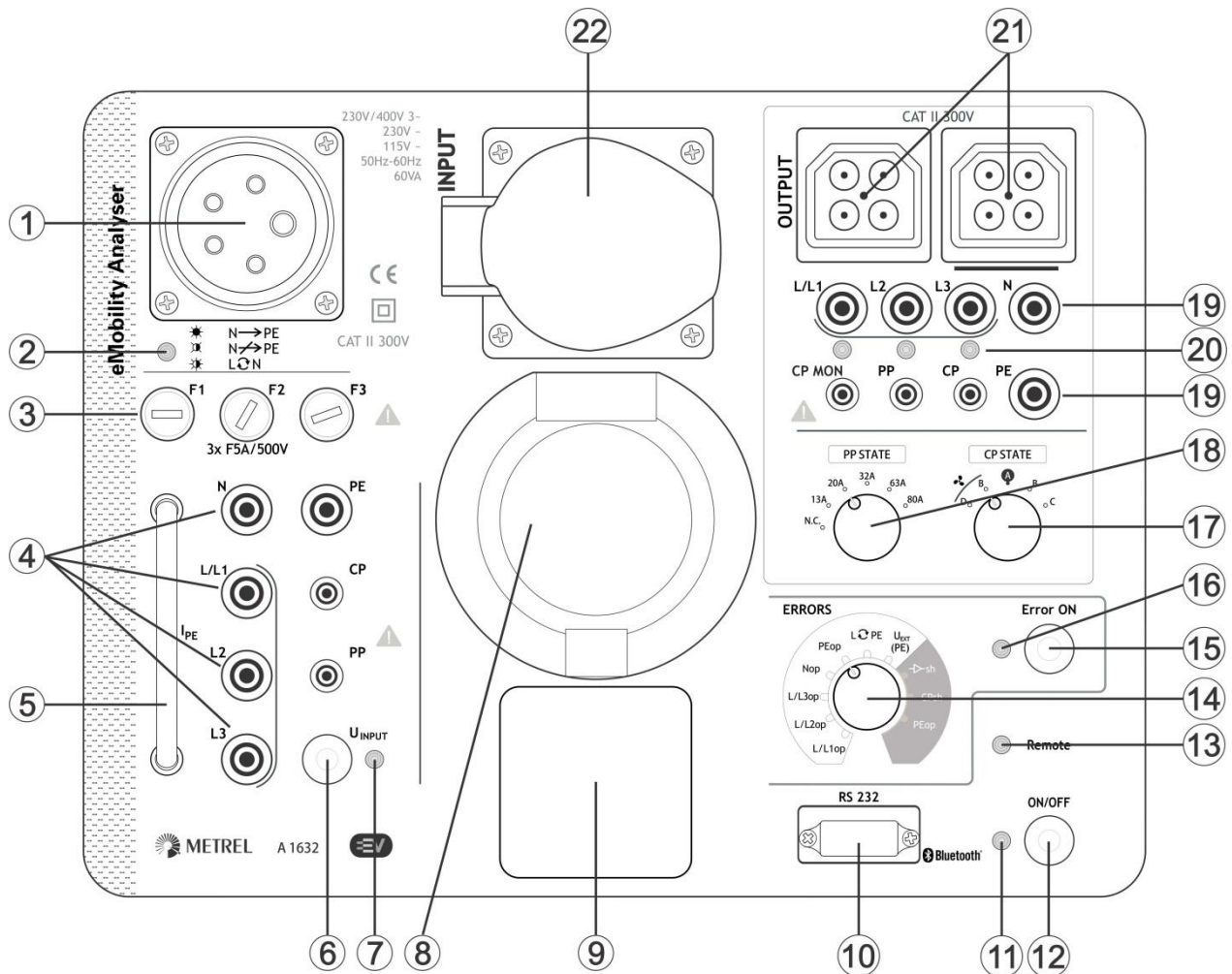
Figure 3.1: Front panel
