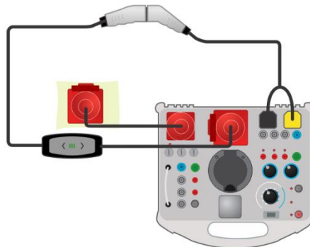
Figure 5.3: Connection of a 3 phase Mode 2 charging cable
